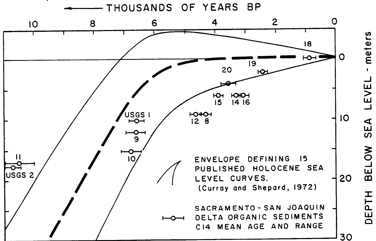
FIG. 4.— Radiocarbon age and depth of Sacramento-San Joaquin Delta sediments compared with a "calibration envelope" of world-wide Holocene sea level curves. Sample locations shown in Figure 2.
