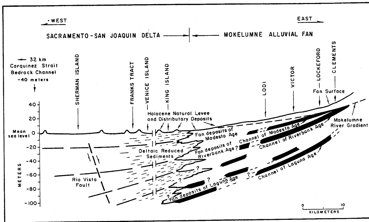
FIG. 3. — Interfingering interglacial deltaic and glacial channel deposits.
